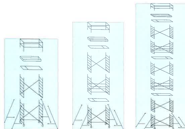
AluLight 1020-S L10-00-2507-0-S
